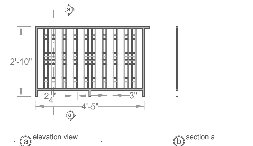
elevation view
