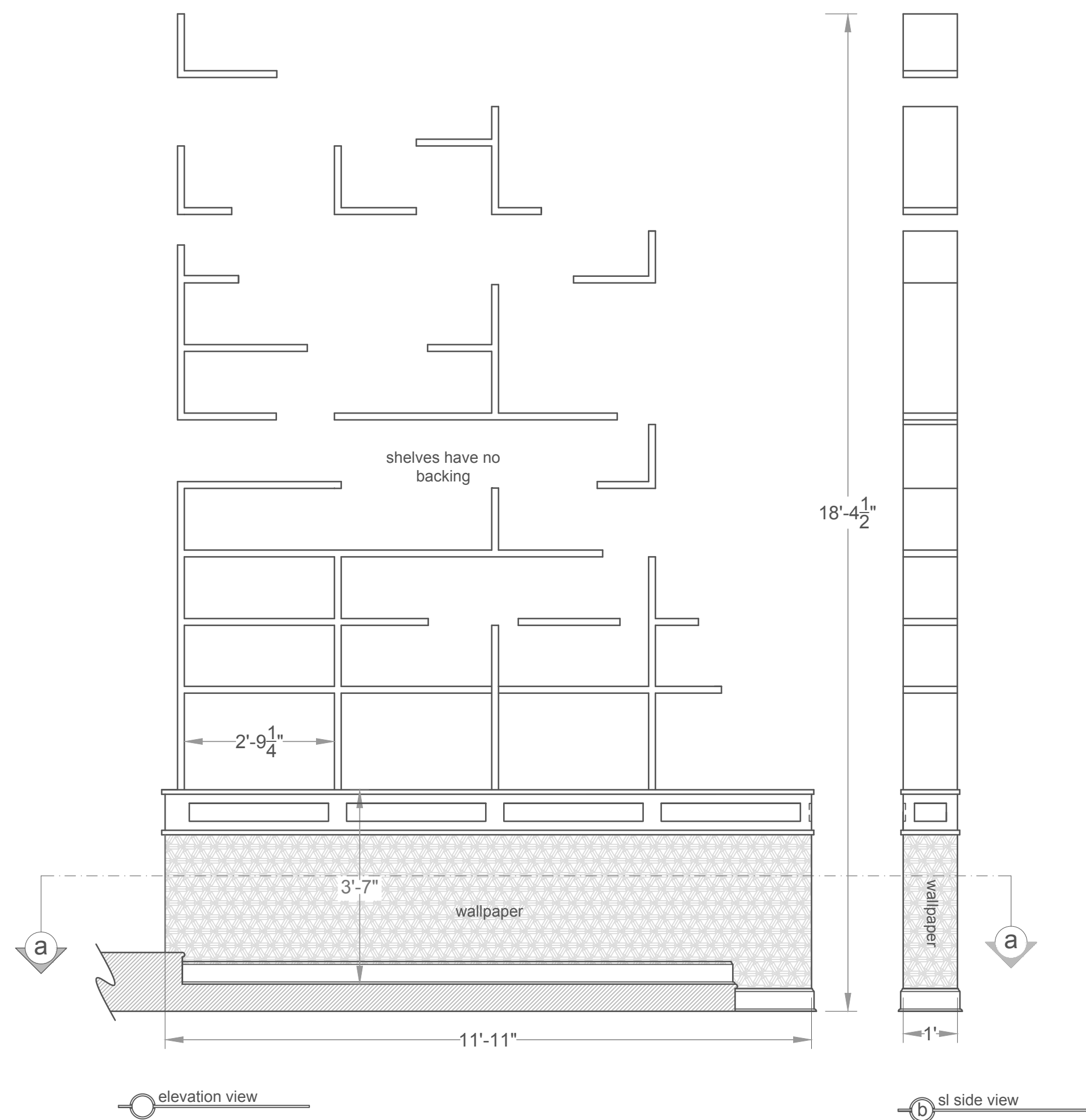
elevation view
